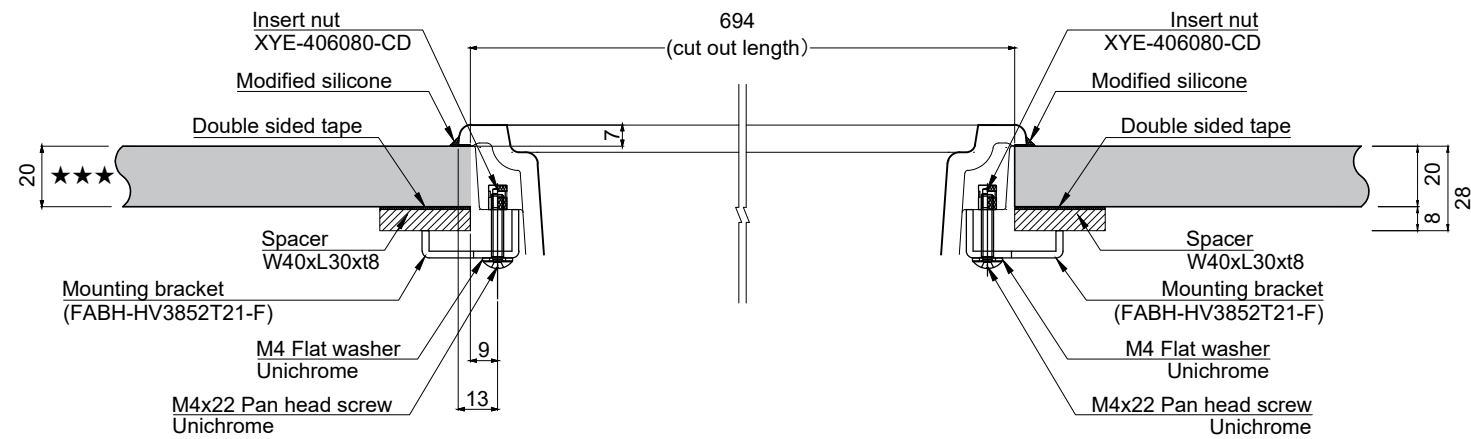
Sec A - A S:1/2.5
