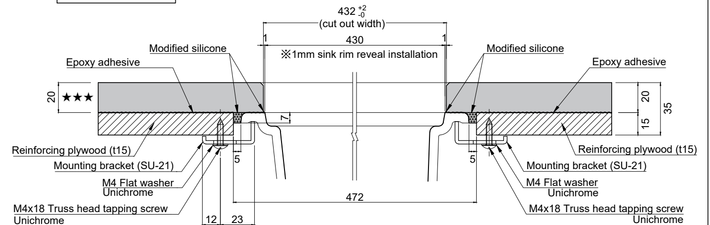
Sec B - B S:1/2.5
