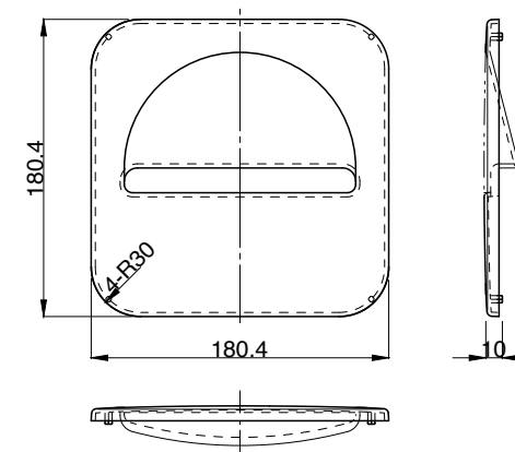
HF180×180 Drain Outlet Stopper
