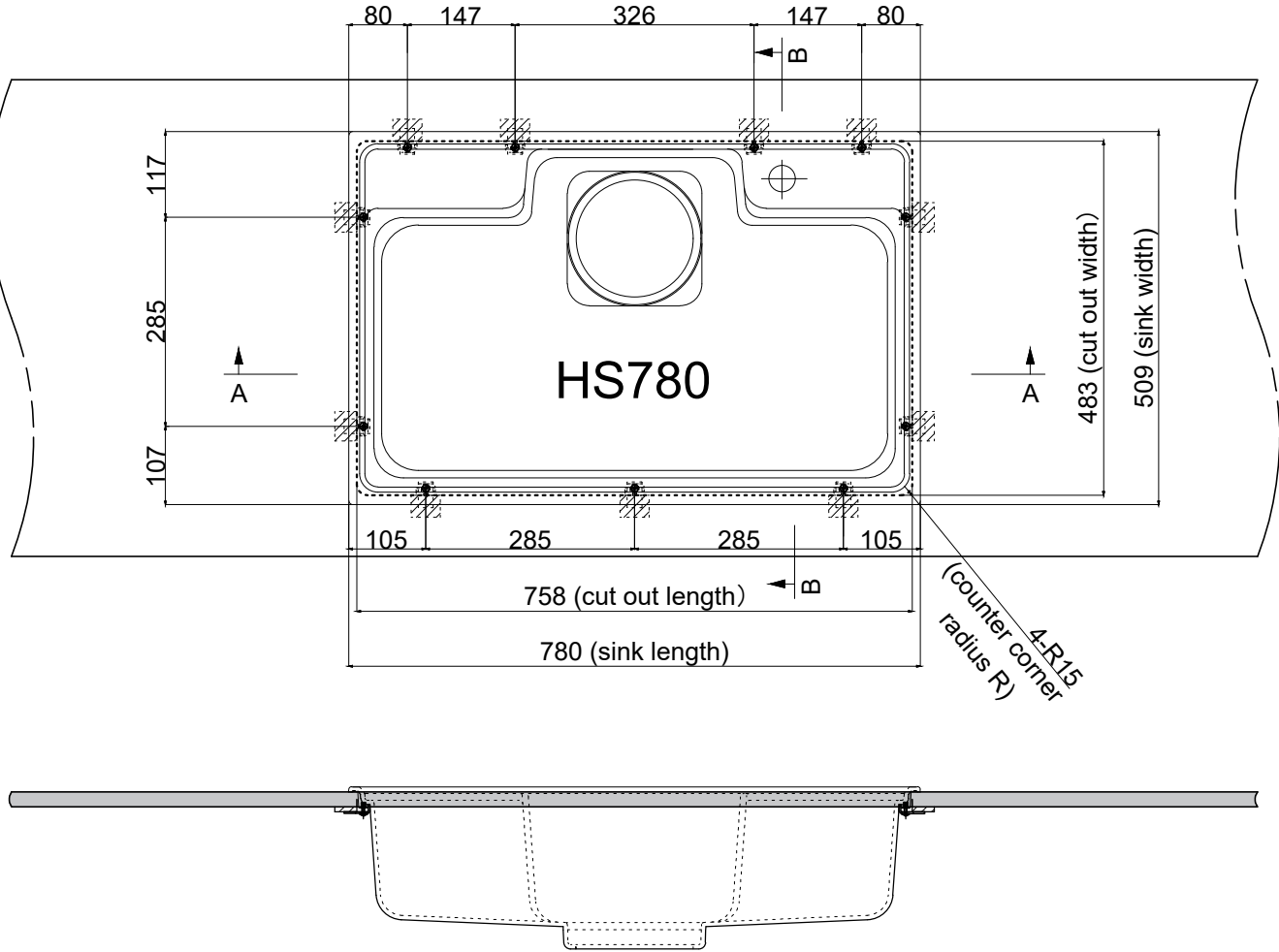
Plan view S:1/10
