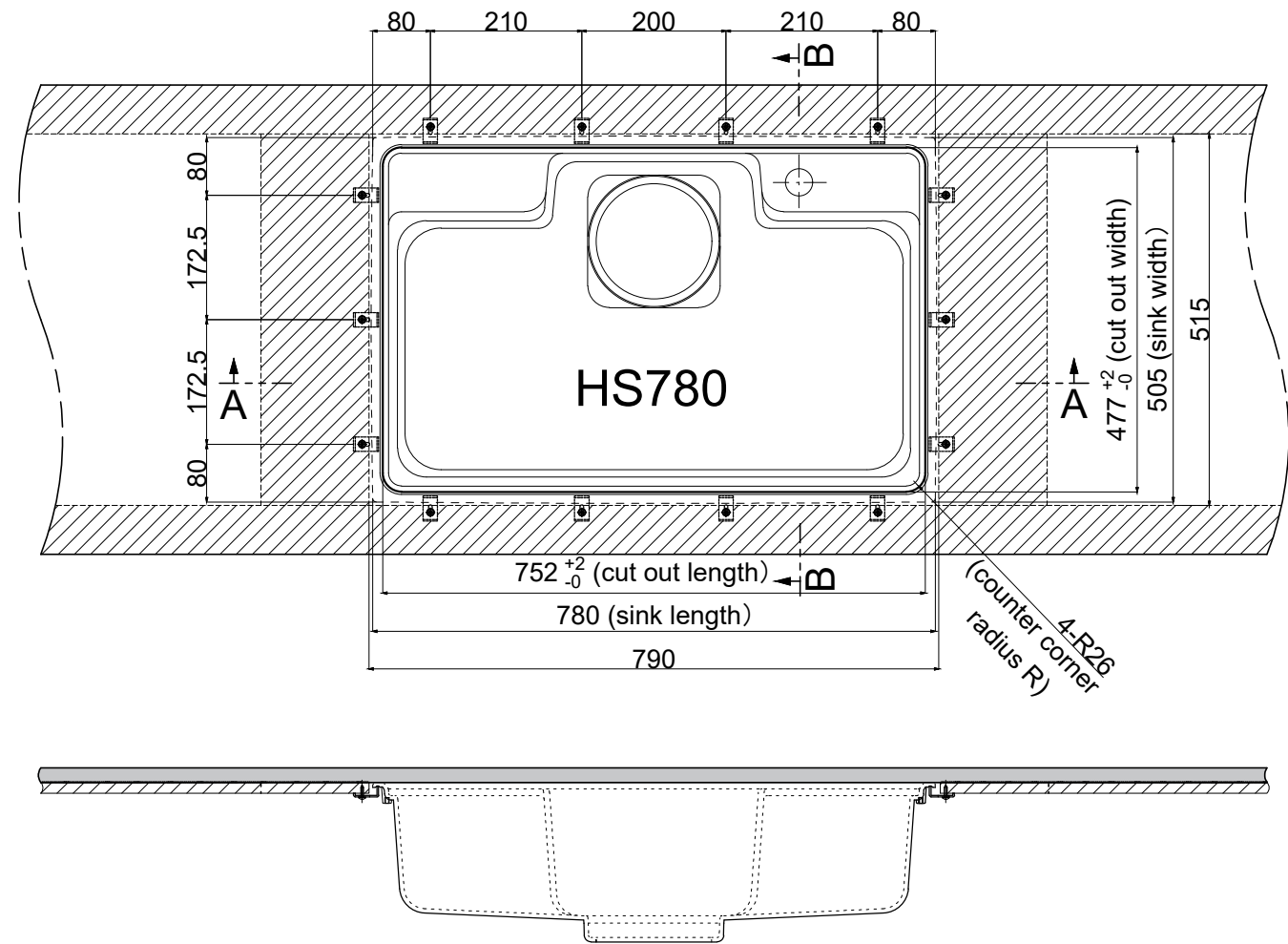
Plan view S:1/10
