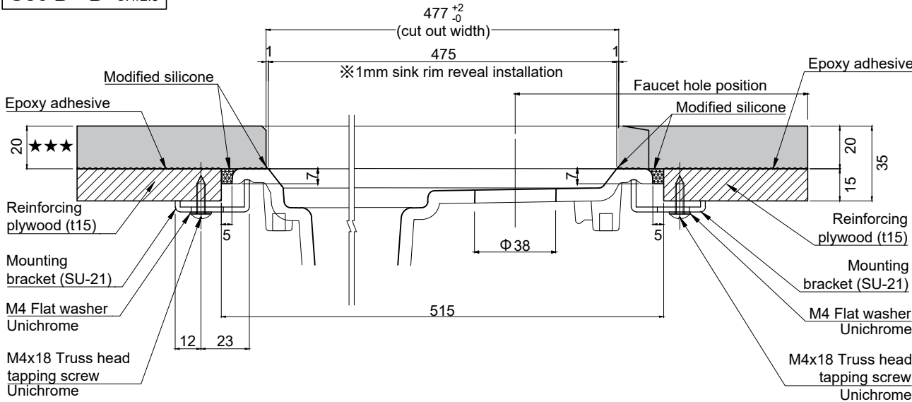
Sec B - B S:1/2.5
