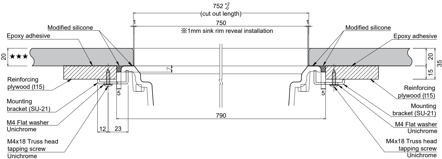
Sec A - A S:1/2.5
