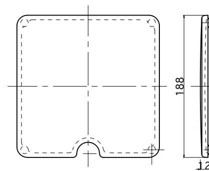
HF188×188 Drain Outlet Stopper
