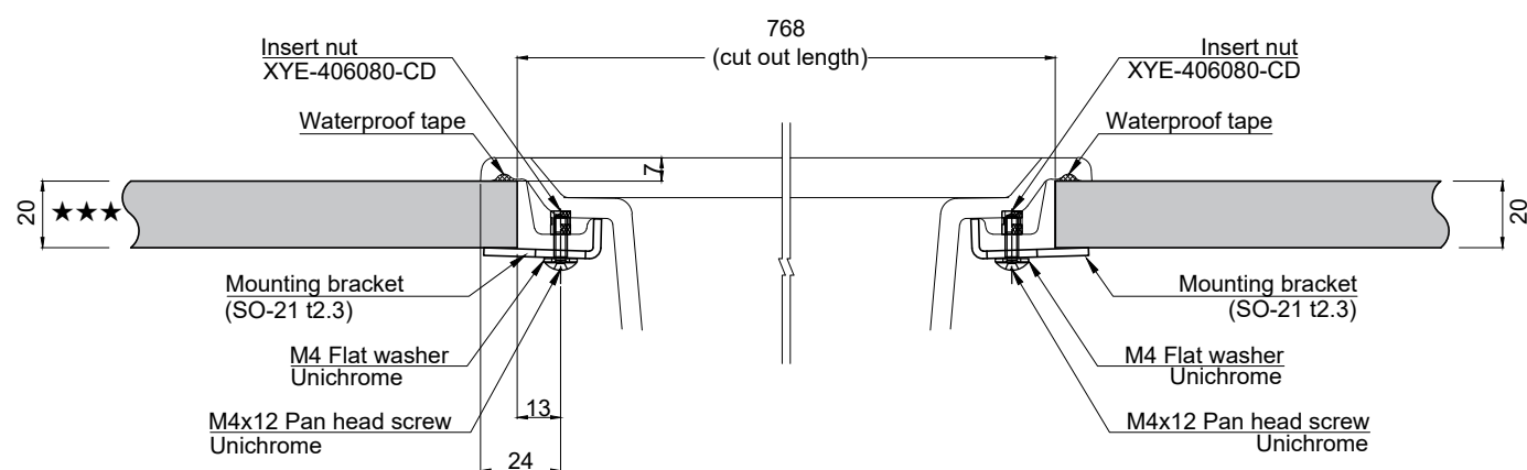
Sec A - A S:1/2.5
