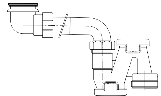
YBΦ302" Hand -Tightening Nut (2" Triangle Packing)
