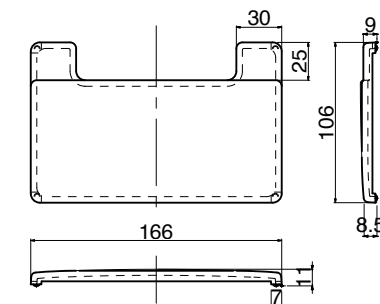
HF106x166 Drain Outlet Stopper
