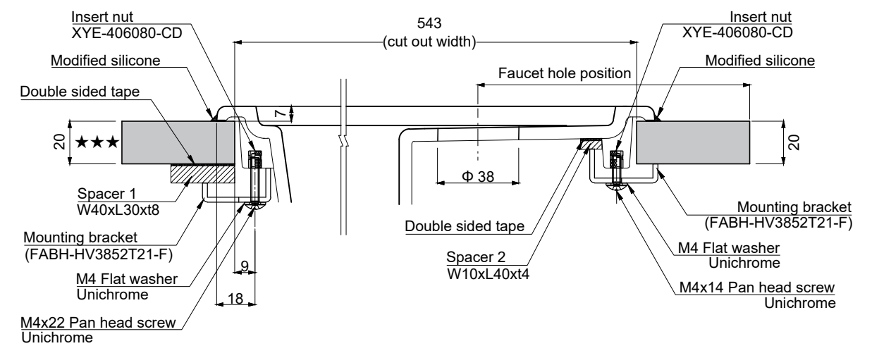
Sec B - B S:1/2.5
