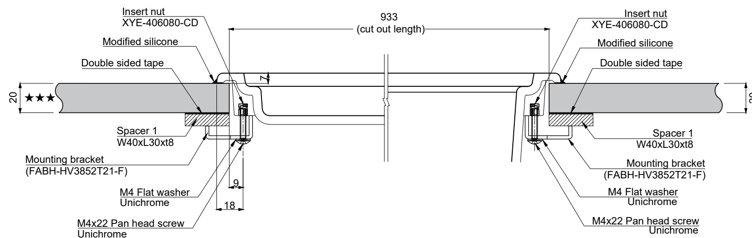
Sec A - A S:1/2.5
