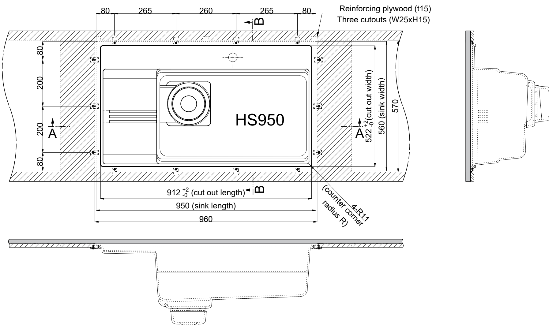
Plan view s:1/10
