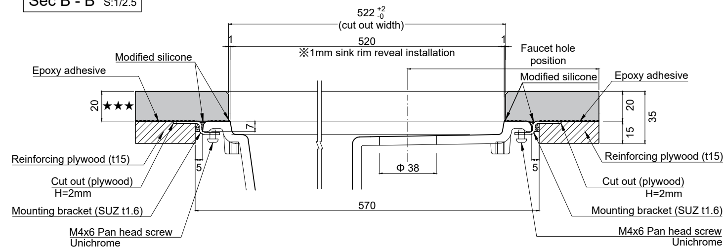
Sec B - B S:1/2.5
