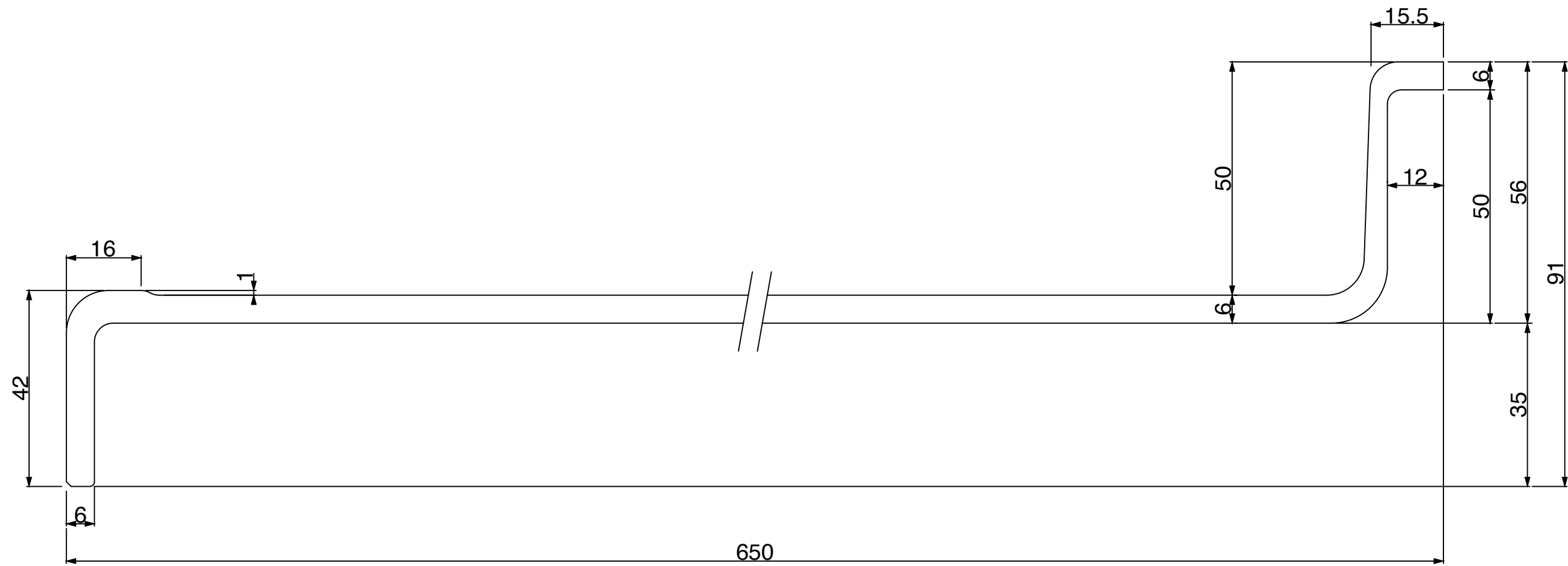
Section (S=1/1)
