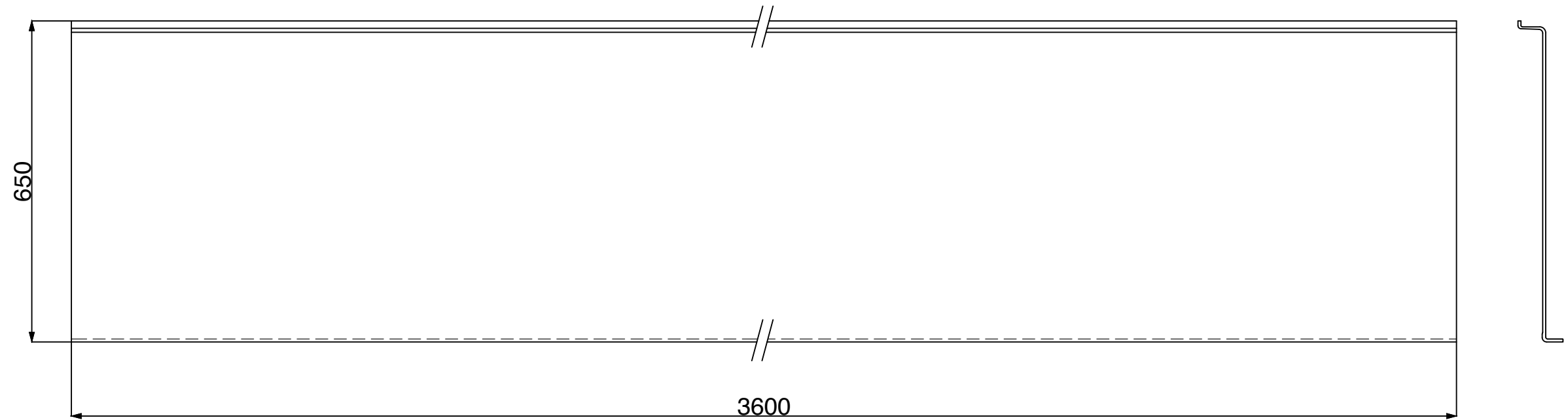
Plan (S=1/10)
