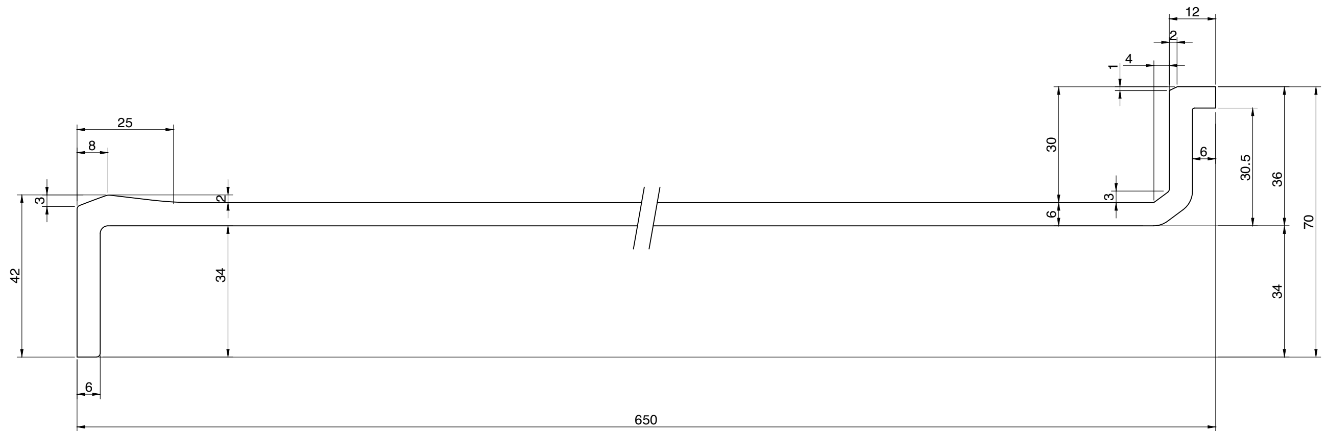
Plan S=(1/10)
