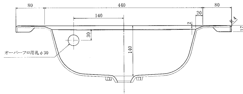
Sec B - B
