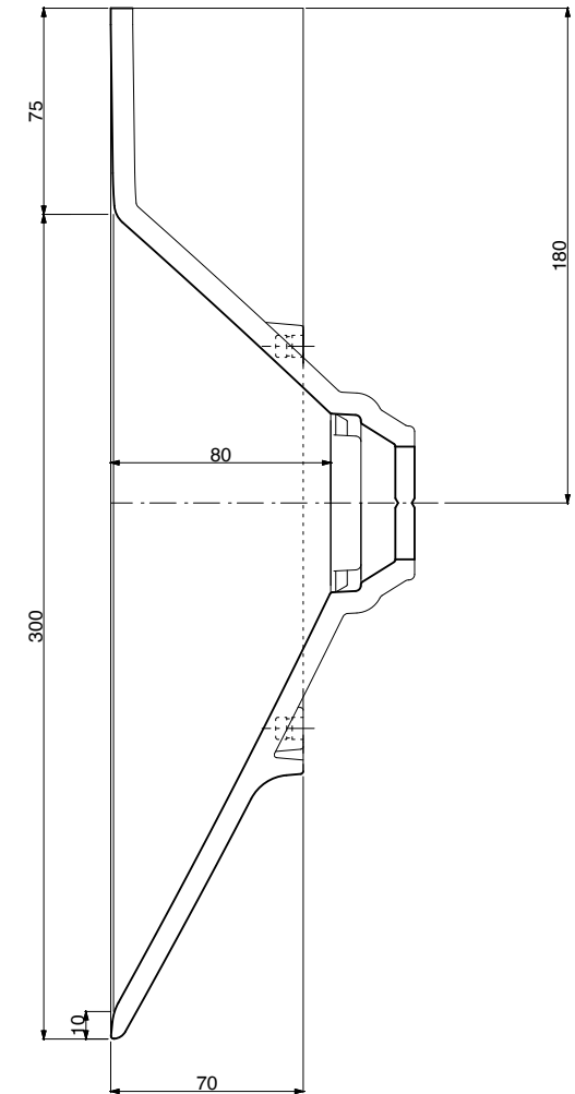
Section B-B
