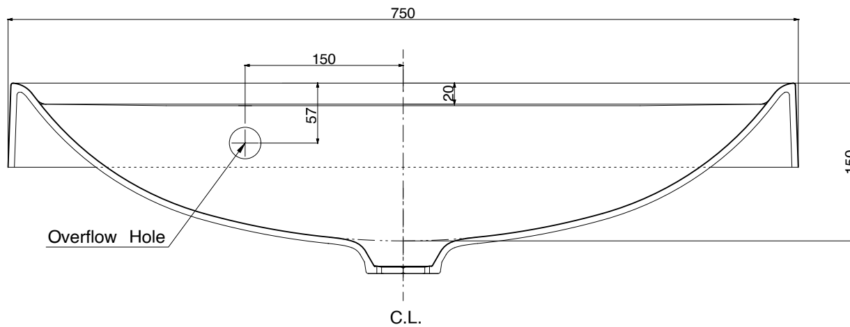
Section B-B
