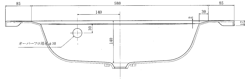
Sec B - B
