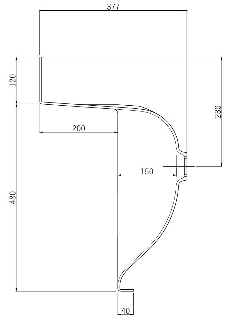
Sec B-B
